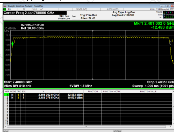
Hopping Seq. NVNT 2-DH5 2441MHz Ant1
