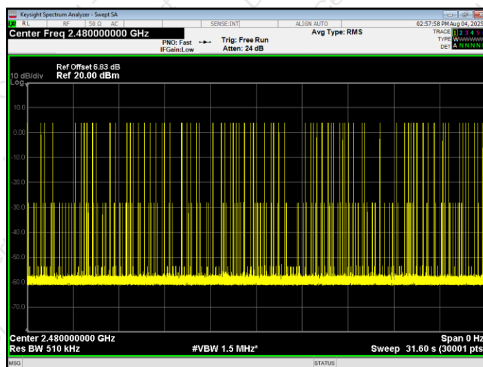
Dwell NVNT 1-DH5 2480MHz Ant1
