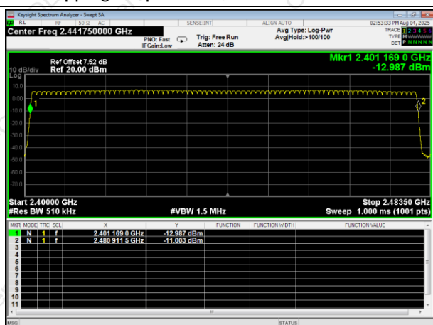
Hopping Seq. NVNT 1-DH5 2441MHz Ant1
