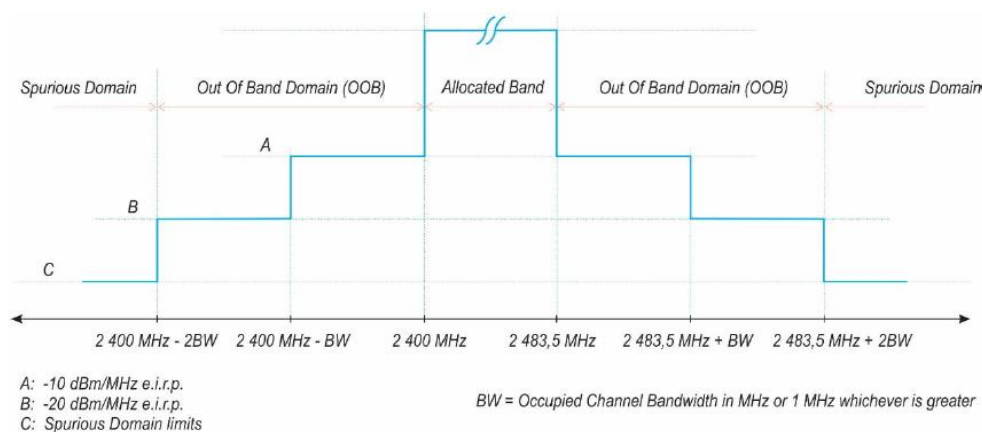
Figure 3: Transmit mask
