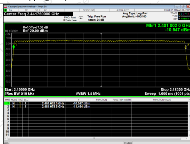
Hopping Seq. NVNT 2-DH5 2480MHz Ant1
