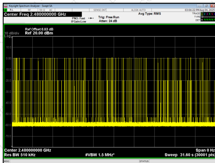
Dwell NVNT 2-DH5 2480MHz Ant1
