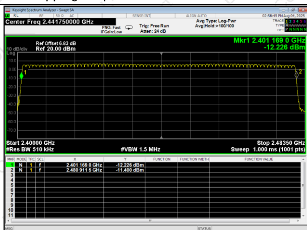
Hopping Seq. NVNT 1-DH5 2480MHz Ant1
